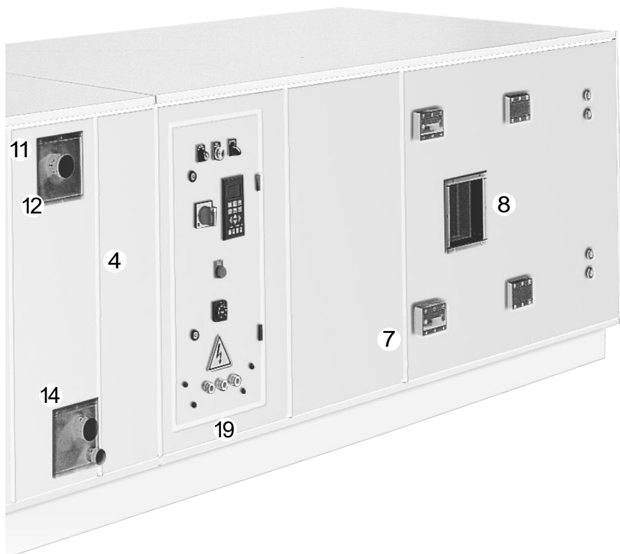
⑦ Seal
