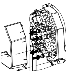
4-pipe version - 4-track valve
